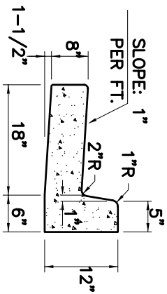
SECTION B-B 18" VERTICAL CURB AND GUTTER (RESIDENTIAL)
